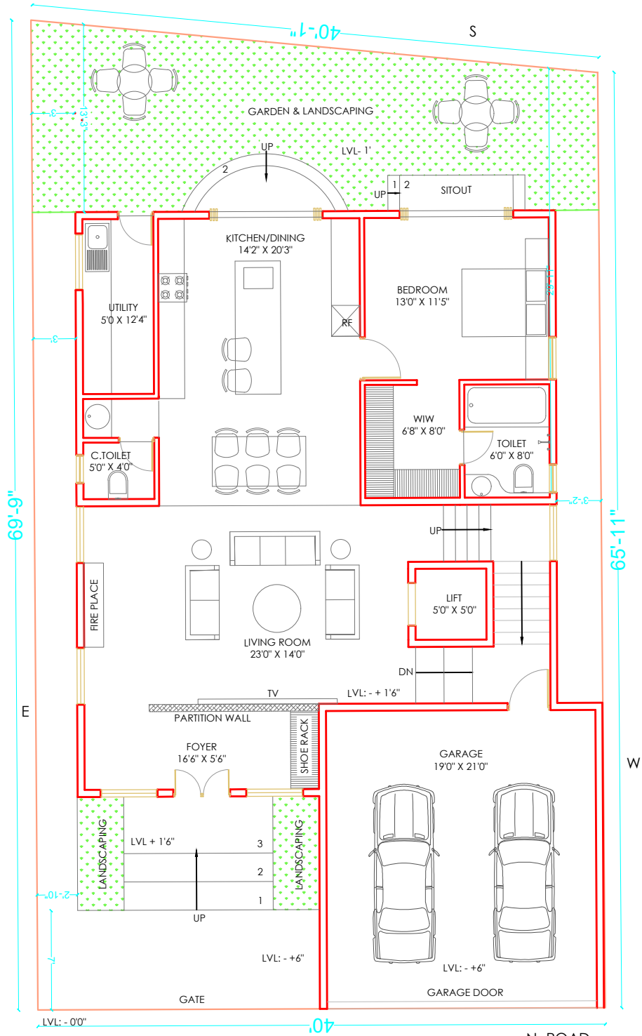
GROUND FLOOR PLAN:- 1717 SFT
