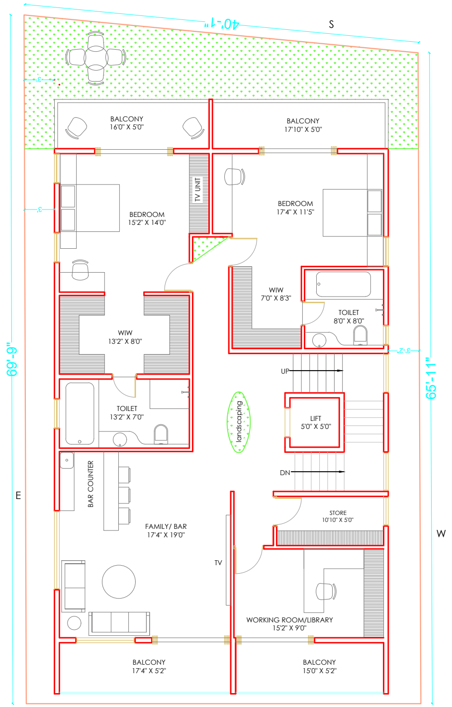
FIRST FLOOR PLAN:- 1703 SFT BALCONIES:- 333 SFT
