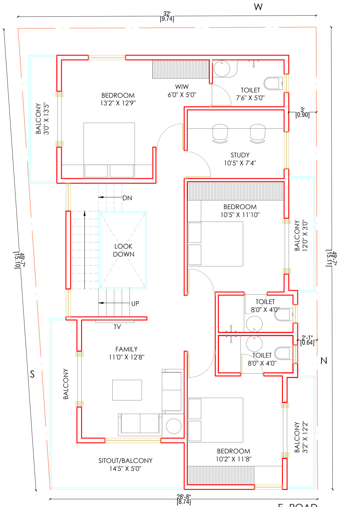
FIRST FLOOR PLAN:- 1053 SFT BALCONIES:- 219 SFT
