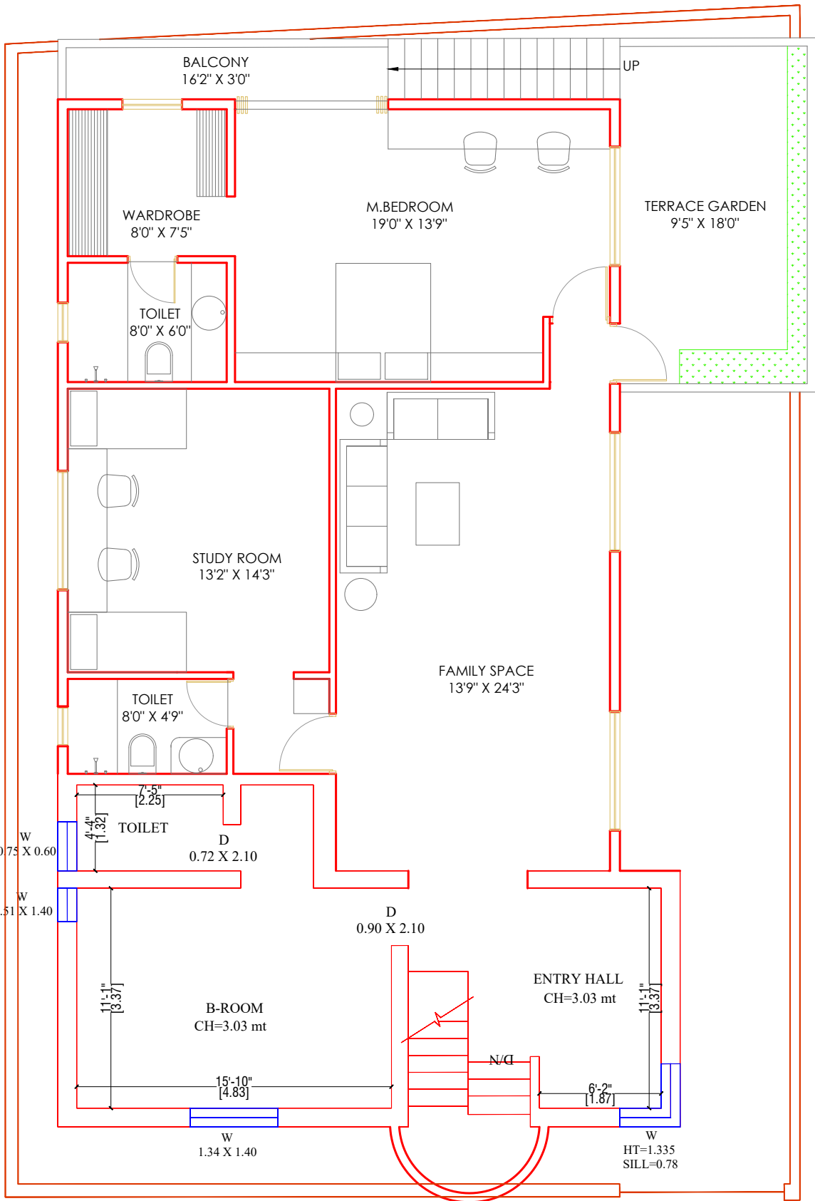
FINAL FIRST FLOOR PLAN:- 1478 SFT
