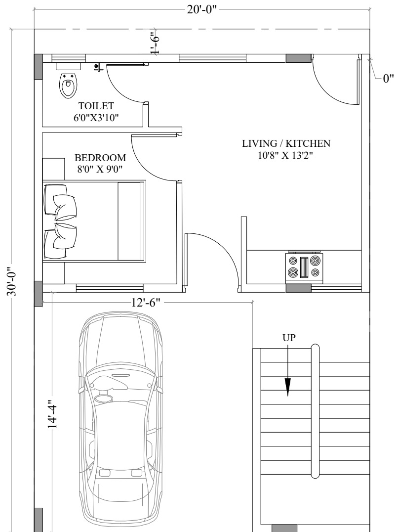
SOUTH ROAD GROUND FLOOR PLAN
