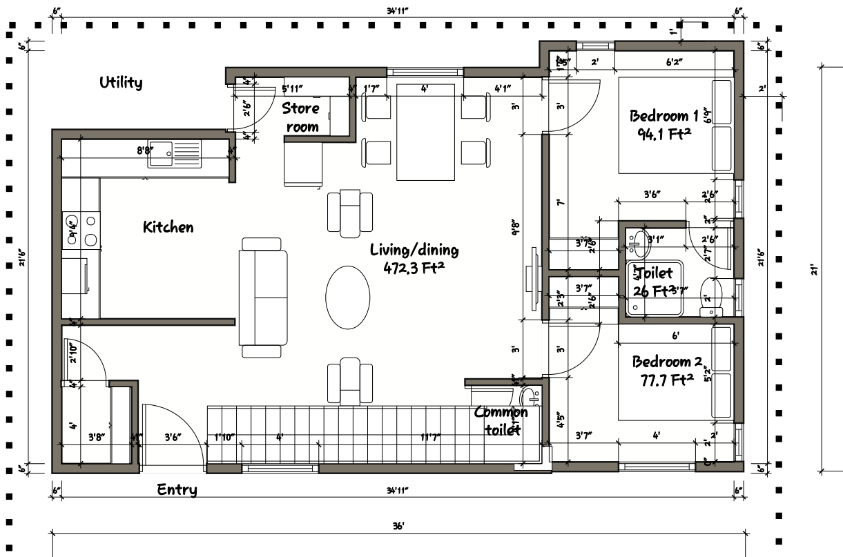
Ground floor Option 1 site dimension 36 ft x 21 ft
