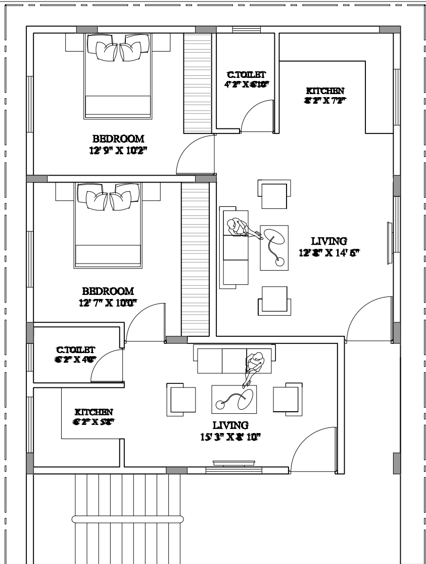
SECOND / THIRD FLOOR PLAN
