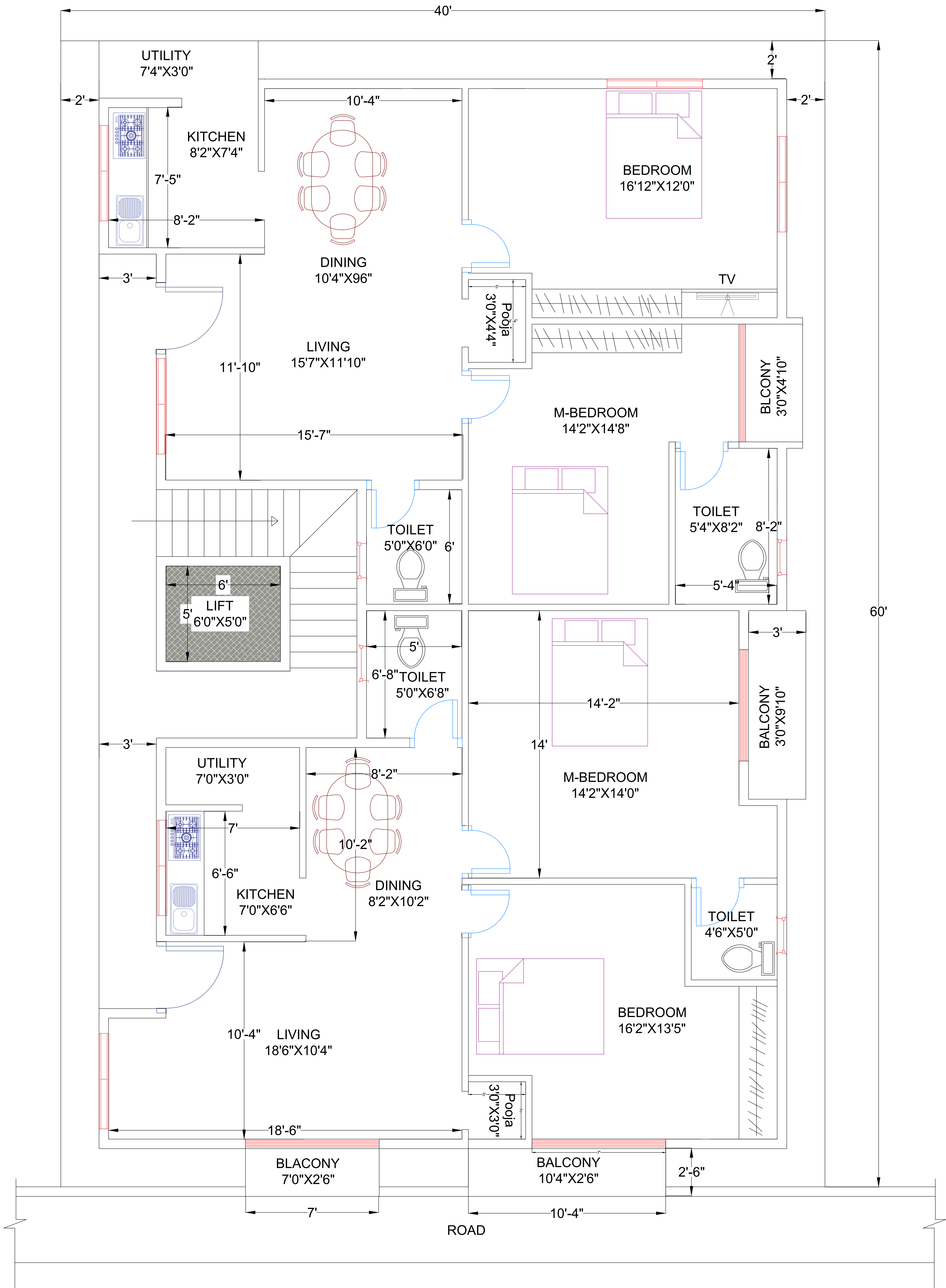
Mr. SUKESH 3rd FLOOR PLAN
