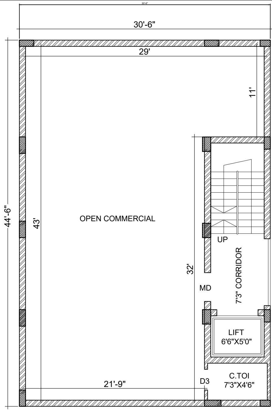
FIRST & SECOND FLOOR PLAN
