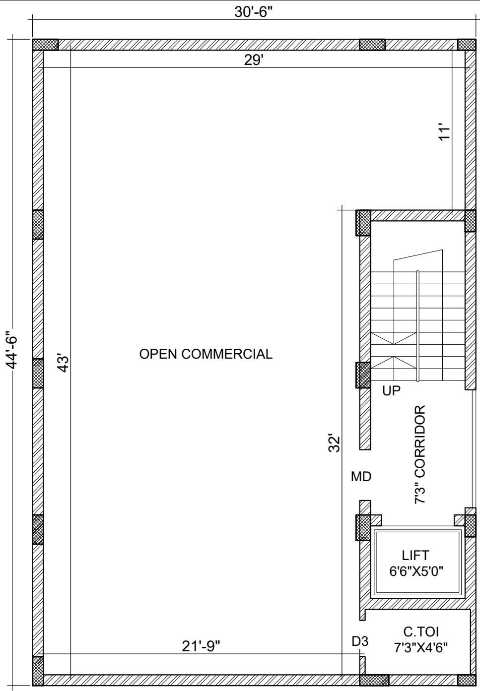
FIRST & SECOND FLOOR PLAN
